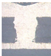
Laser microvia in FR27-0050-40 as performed by Hughes Circuits
