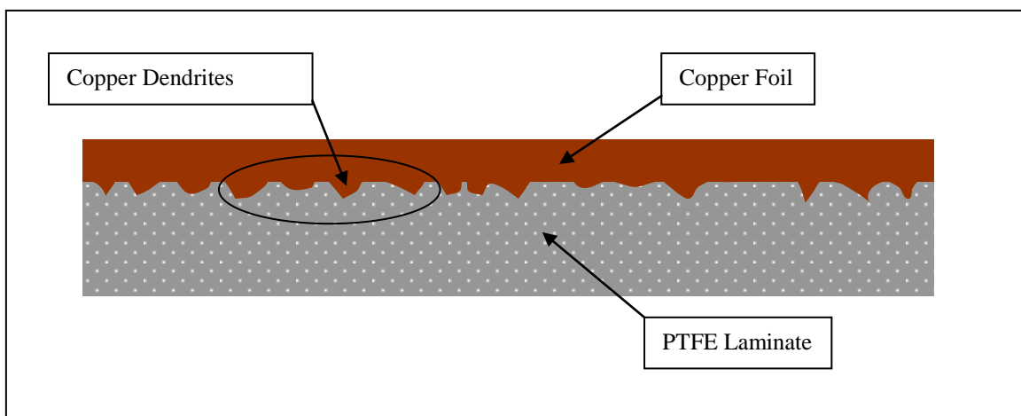
Figure 2 – Illustration of copper laminated to PTFE surface.
