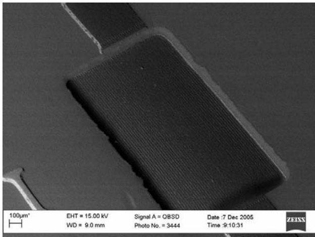
Figure 1 – Cavity in TacLamPLUS.
