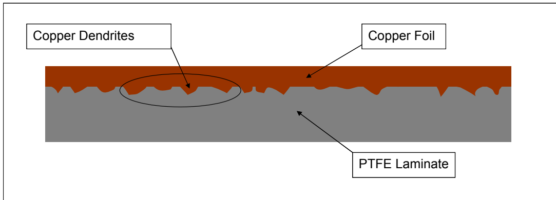
Figure 3 – Illustration of copper laminated to PTFE surface
