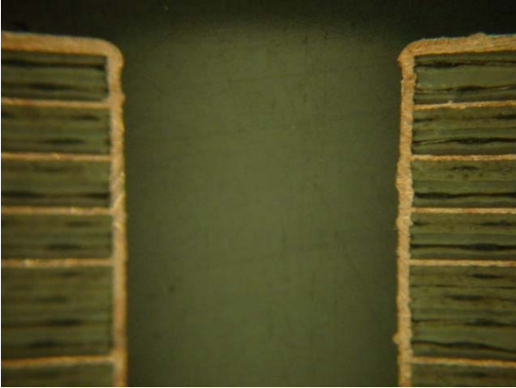
Figure 1 - Multilayer board made with TSM-30 and TacLam TPG-32
