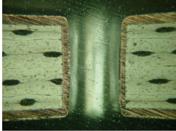
Figure 2 - A typical TSM-30 plated through hole
